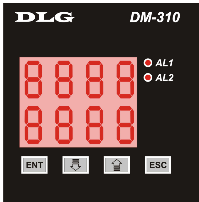
Figura 1 - Painel frontal
