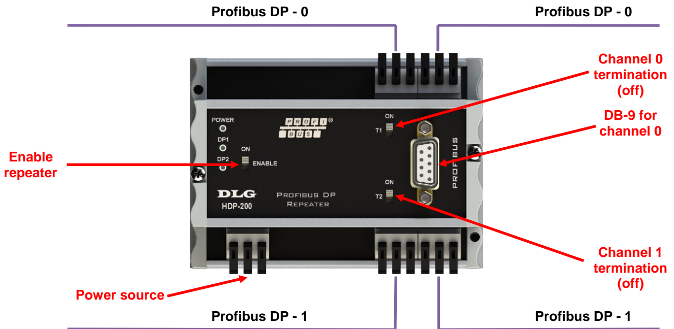
Figure 4 – Installation without termination
