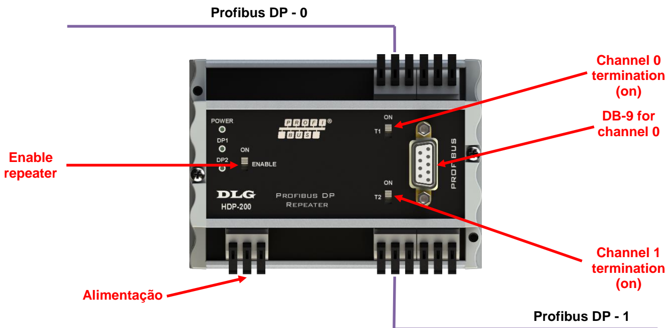
Figure 5 – Installation with termination
