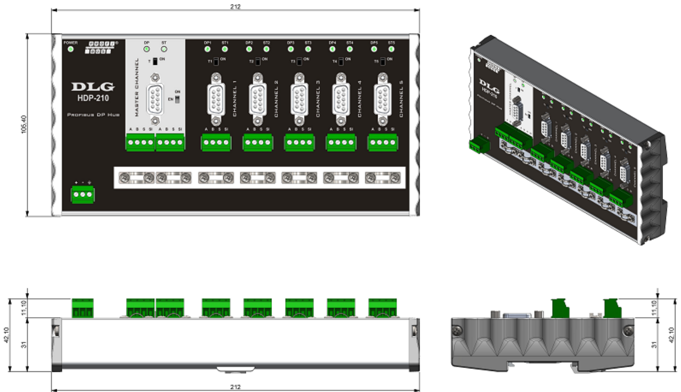
Figure 2 - Dimensions for assembly (in millimeters)
