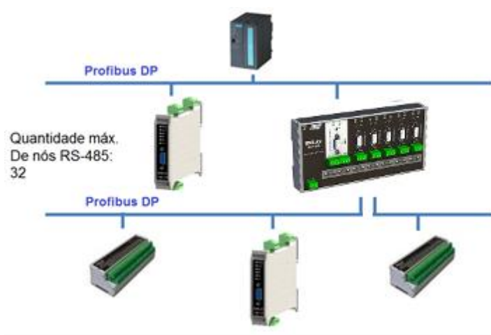
Figure 1 - HDP-210 Application.
