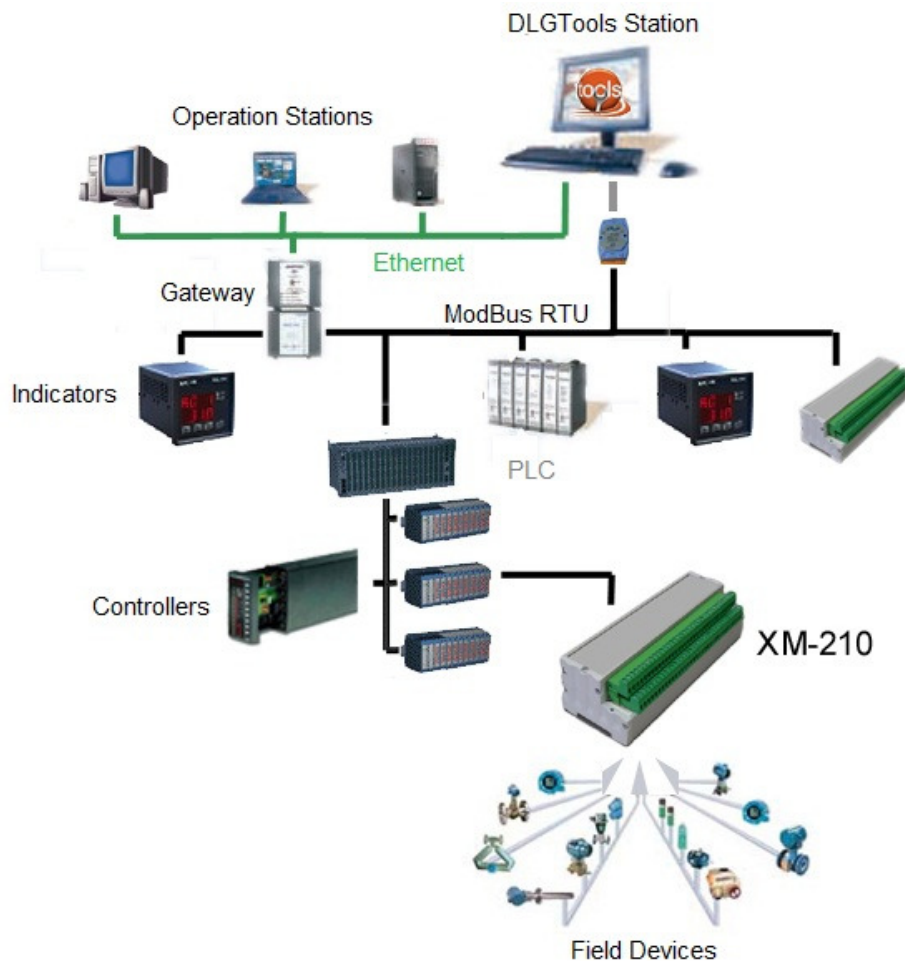
Figure 2 – Modbus network topology with the XM-210
