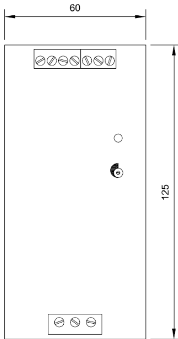
VISTA FRONTAL
