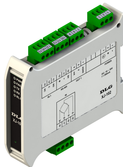
Figura 1 – Conversor XJ-102
