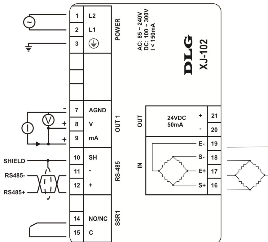
Figura 4 – Borneiras XJ-102/AC
