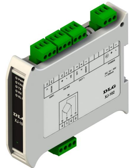
Figura 1 – Conversor XJ-102
