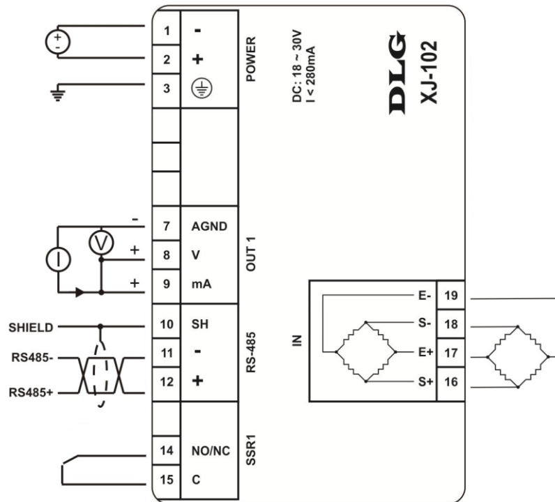
Figura 5 – Borneiras XJ-102/DC
