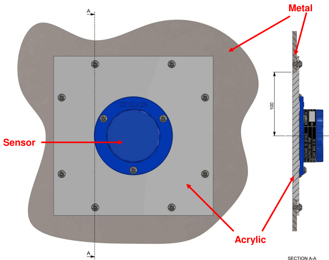
Figure 2 - SC-500 Installation
